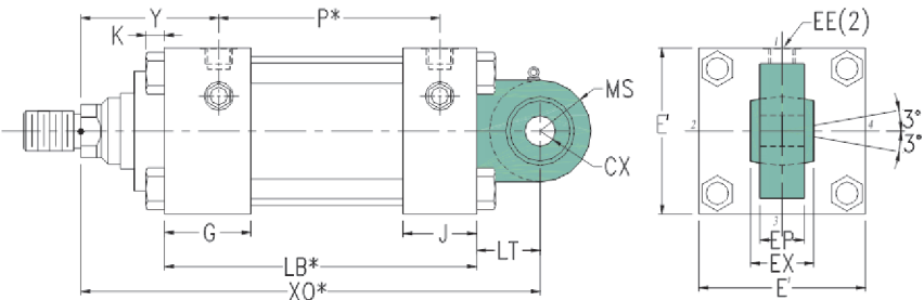
Cap Spherical Bearing (ISO MP5)
