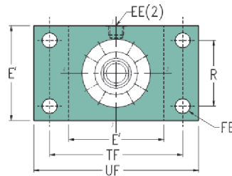
Head Rectangular (ISO ME5)
