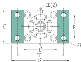
Cap Rectangular (ISO ME6)
